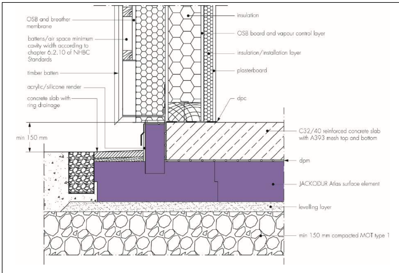
Figure 2 Example of raft foundation reinforced with steel mesh A393 with timber framed wall
