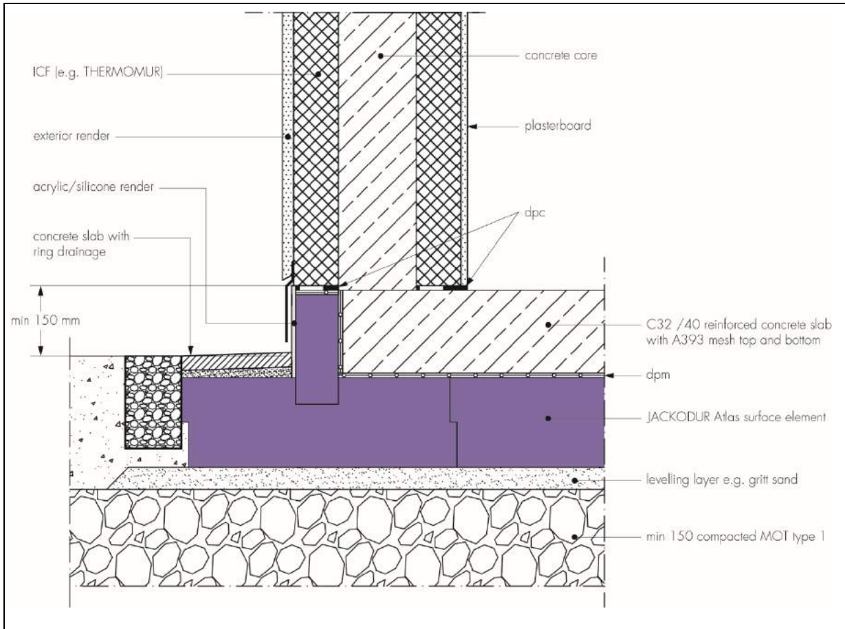
Figure 3 Example of Insulated Concrete Form (ICF)
